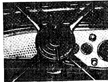
Fig. 12. The lighting switch control is at the hub of the steering wheel.
