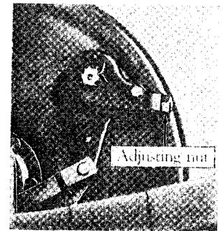
Fig. 25. A temporary brake adjustment can be secured by turning the adjusting nut on each brake clockwise one-half turn. The front brake is shown above at the left, the rear brake at the right.
