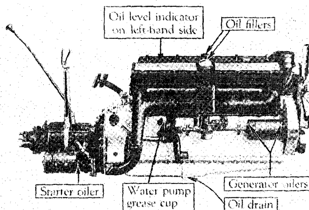
Fig. 22. Showing the location of the oil filler, oil level indicator, oil pan drain plug and other lubrication features.
