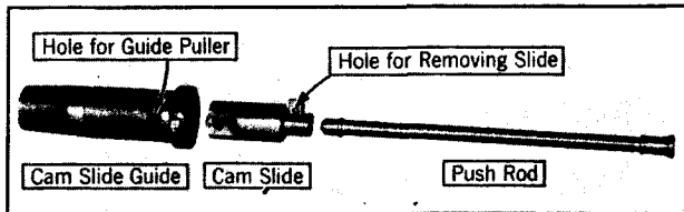
Fig. 32. The cam slides and guides can be removed without taking off the cylinder blocks.
