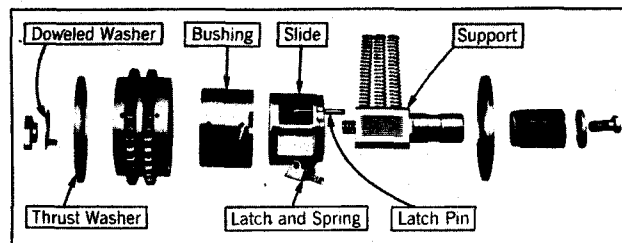
Fig. 36. Exploded view of the automatic chain adjuster.
