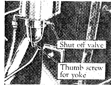
Fig. 24. The two gasoline filters should be removed and cleansed regularly.
