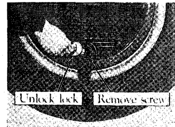
Fig. 18. To remove a spare tire, unlock the lock, remove the screw and take off the clamp.
