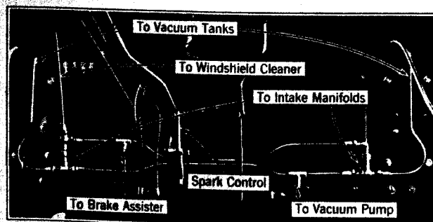
Fig. 44. The driver's side of the dash with the rear dash cover removed.
