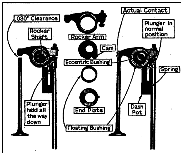
Fig. 34. At the left the plunger is held all the way down to show the clearance. At the right, the plunger has turned the eccentric bushing to take up this clearance.
