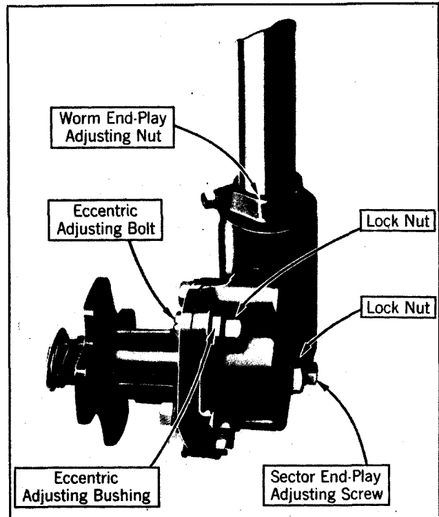
Fig. 41. Be sure all adjustments are made exactly as directed.
