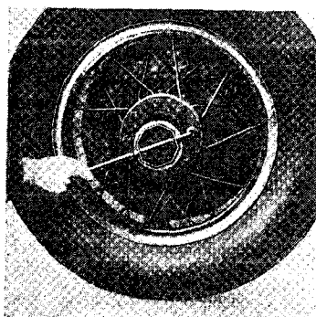
Fig. 19b. Jack up the axle until the weight of the car is off of the wheel, but with the tire still dragging. Loosen the cap screws around the wheel hub by turning them in a counter-clockwise direction with the wrench. Then jack the wheel up further, remove the cap screws and take the wheel off of the hub.
