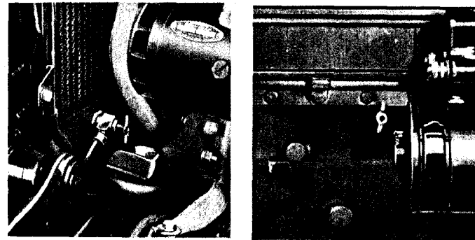
Fig. 18. Both valves must be opened in order to drain the cooling system thoroughly.
