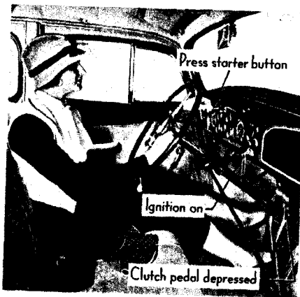
Fig. 9. The starter button is on the instrument panel. There is no hand choke control.
