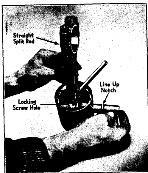
Fig. 8. Assembly of 38-90 piston and connecting rod
