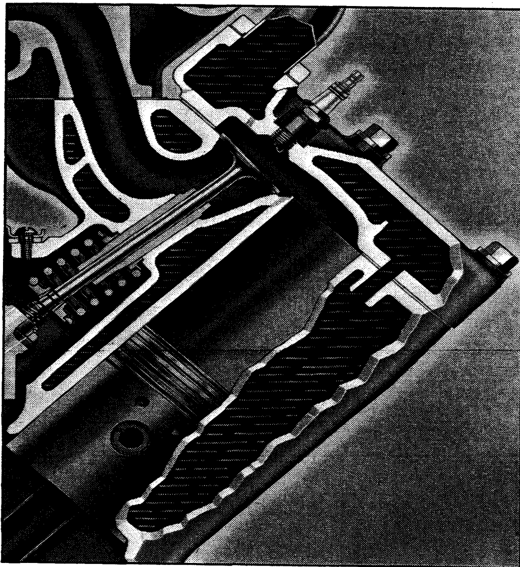
Full Length Water Jackets
