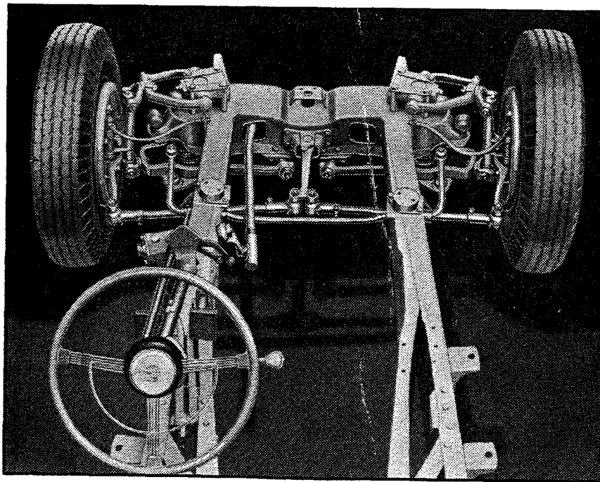
Fleetwood V-8 Center Point Steering System
