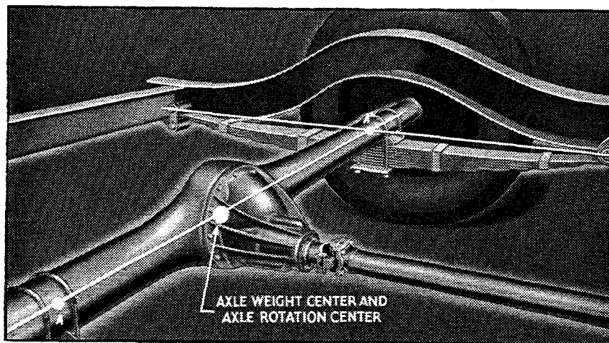
Cadillac-LaSalle Hi-Plane Hotchkiss Drive
