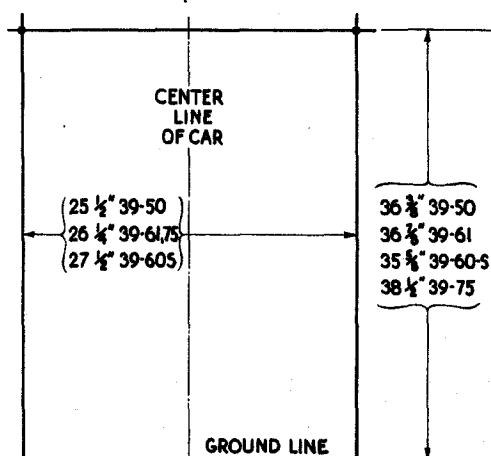
Fig. 18. Dimensions of headlamp center locations.
