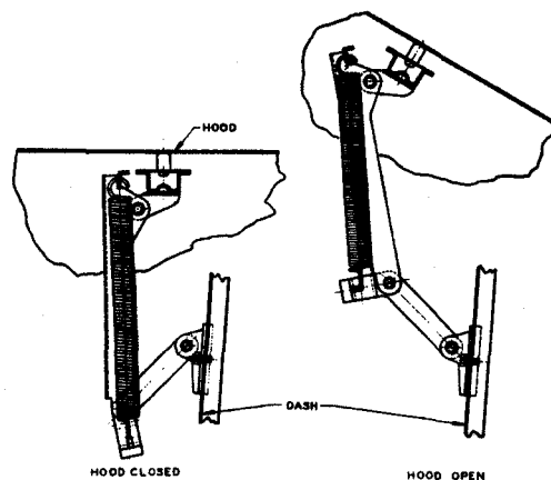
Fig. 16. Hood support bracket, Series 39-50 and 61.
