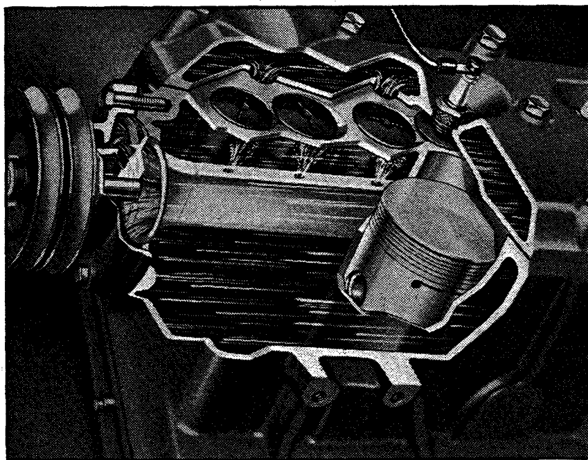
Positively Cooled Valves and Full Length Water Jackets
