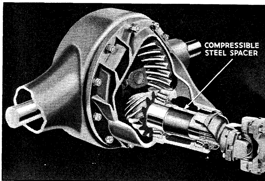
Cadillac-LaSalle Precision-built Hypoid Rear Axle
