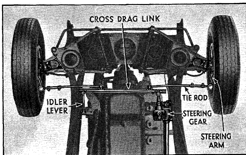
Parallel Cross Steering—LaSalle and Cadillac "61"
