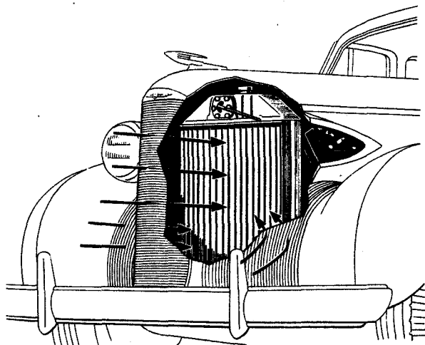
Fig. 21. Flow of air through radiator grille and side grilles (39-50 shown).
