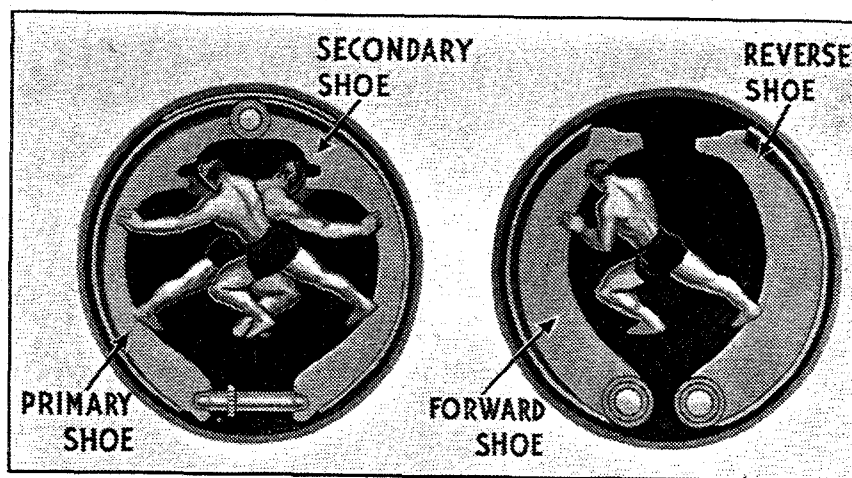
With Self-Energization, Both Brake Shoes Are Effective
