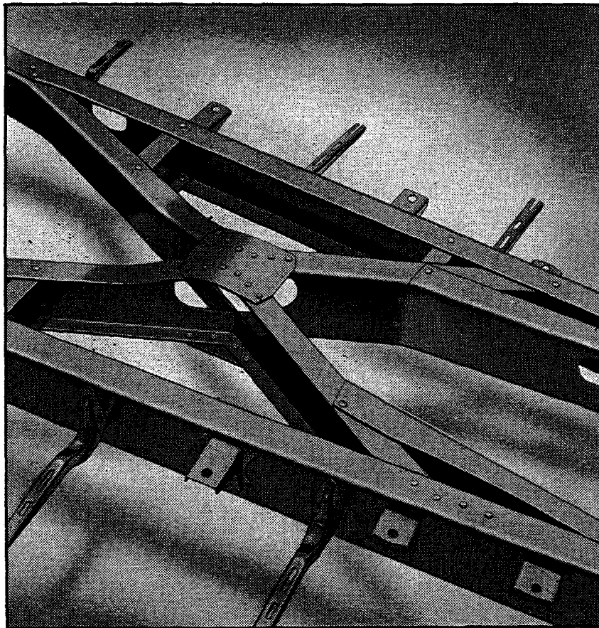
Rigid Frame Bracing and Deep Center Junction
