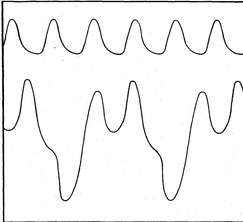
(Above) Sixteen Torque Curve (Below) Typical 12 Torque Curve
