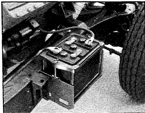
Cadillac Battery Location Illustrated on the "61" Chassis
