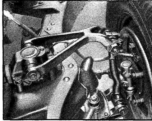
End-to-End Type Shock Absorbers on LaSalle and "61"
