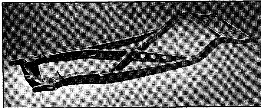
New LaSalle Double Drop Rigid X, I-Beam Frame
