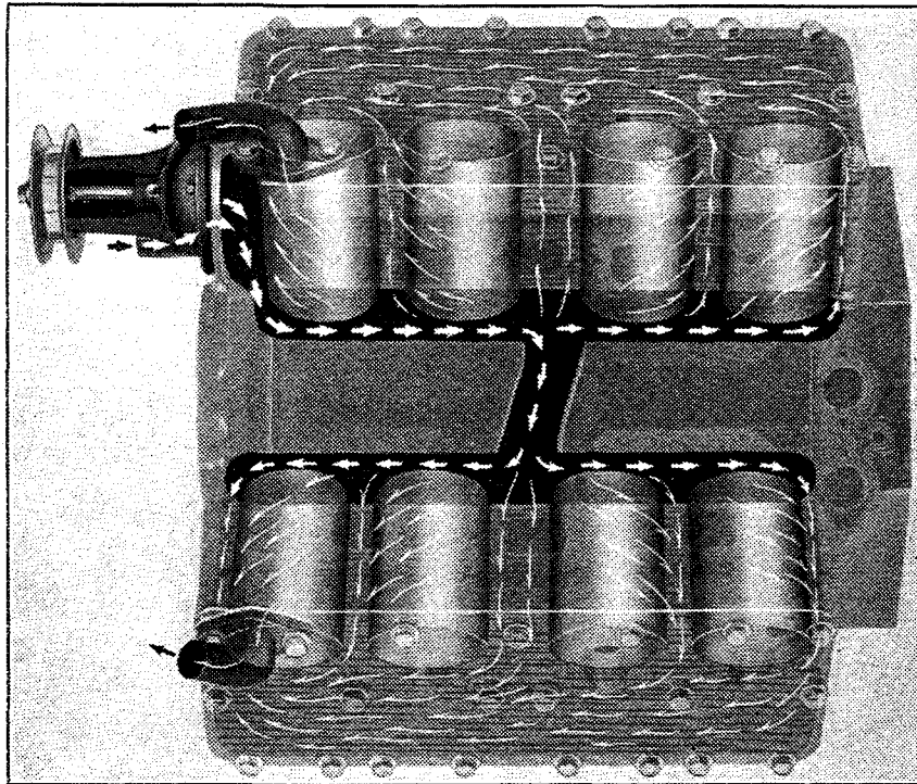
Complete and Uniform Water Circulating System
