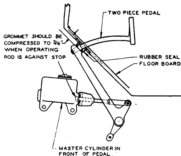
Fig. 5. Brake pedal layout and adjustment, Series 39-50 and 61.
