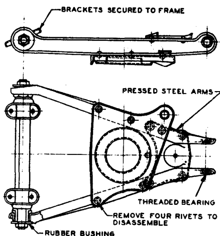
Fig. 2. Lower suspension arm, Series 39-50 and 61.
