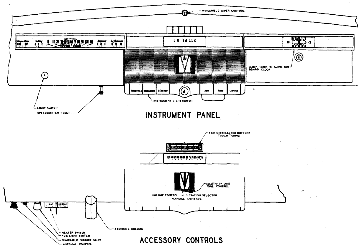
Fig. 20. Diagram of instrument panel and accessory control mountings.
