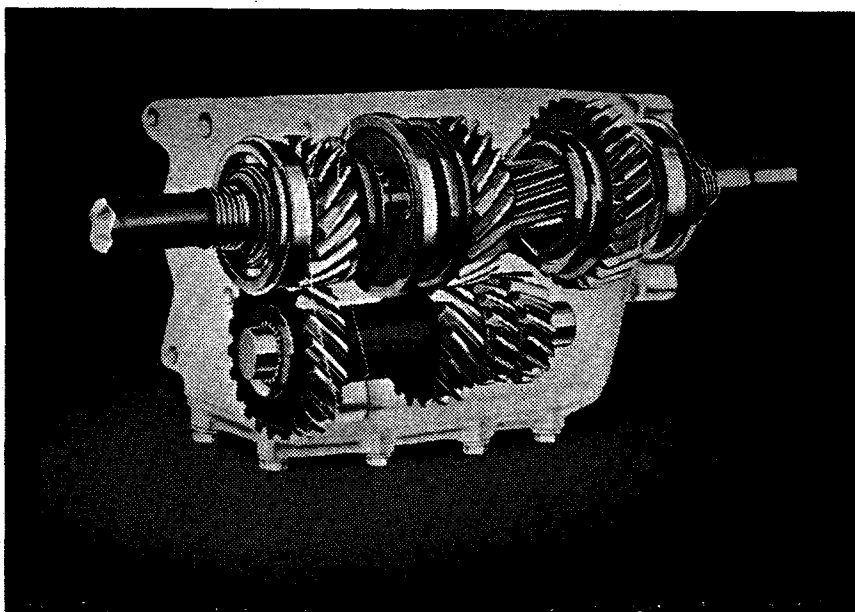
Improved Cadillac Syncro-Mesh Transmission
