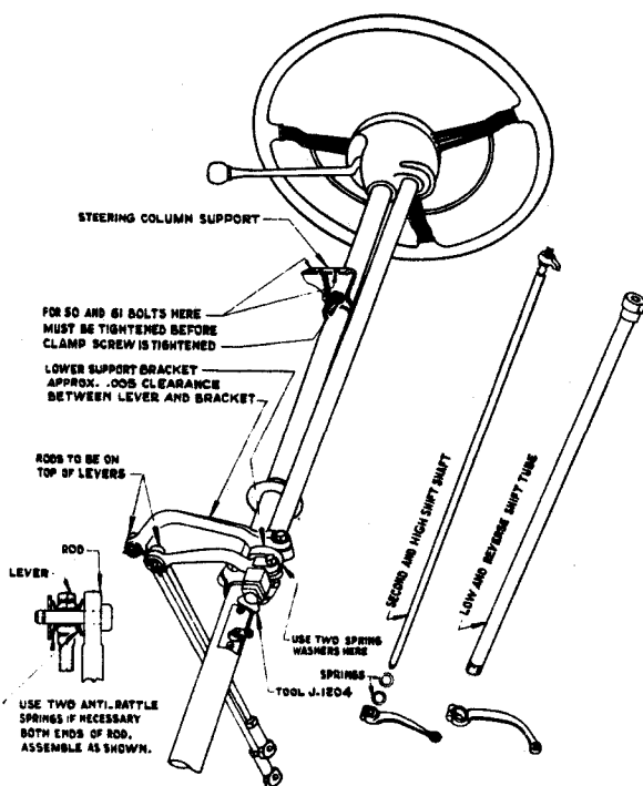
Fig. 11. Shifting mechanism on steering column.
