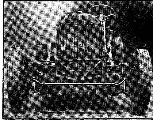
Torsion Shaft Front Stabilizer— LaSalle and "61"
