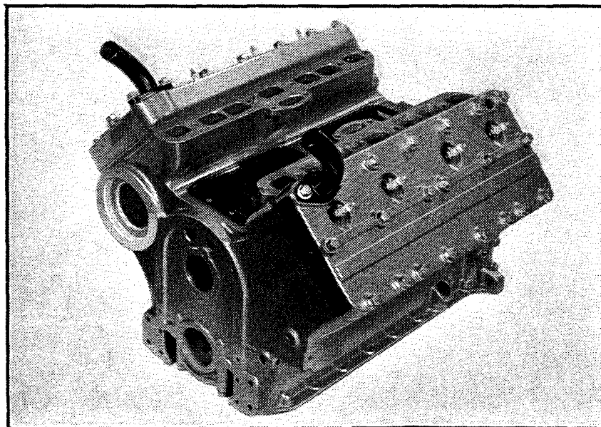
V-9 Enbloc Cylinder and Crankcase
