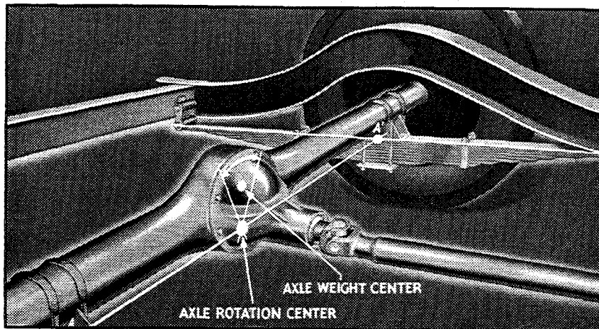
View from above: Conventional Rear Suspension
