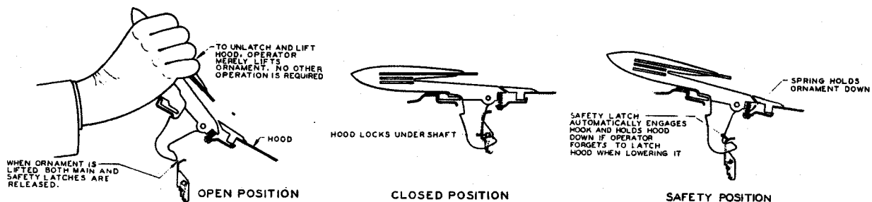
Fig. 17. Operation of hood latch, Series 39-50, 61, 60S and 75.
