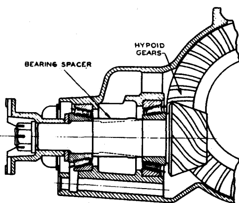
Fig. 3. Cross section of rear axle pinion.
