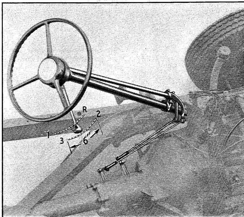
Syncromatic Shift Control
