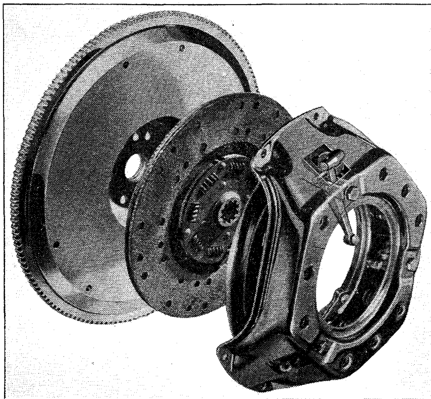
Improved Semi-Centrifugal Clutch for LaSalle
