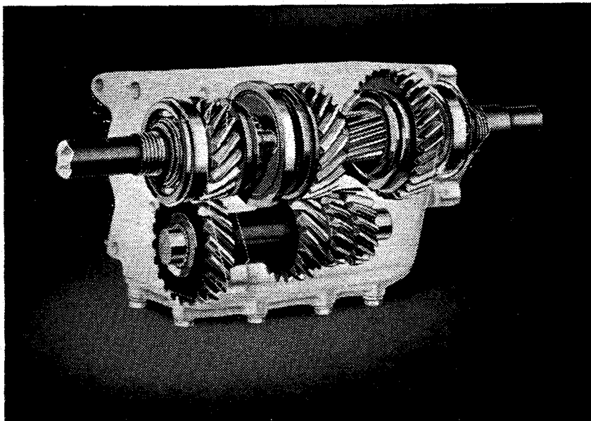
Improved Syncro-Mesh Transmission
