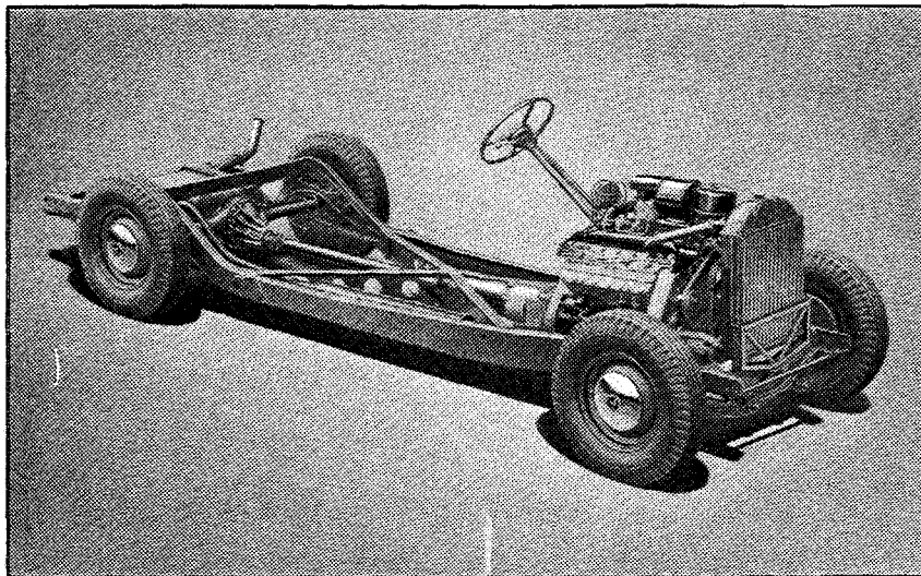
New LaSalle V-8 Chassis
