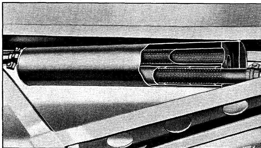
Cutaway View of New Corrosion Resisting Muffler
