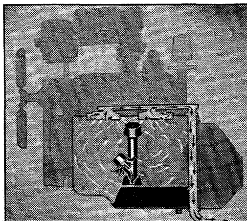
New Crankcase Ventilation System
