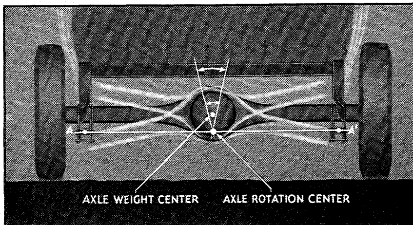
The axle rotation center is below the axle weight center in all conventional rear suspensions.
