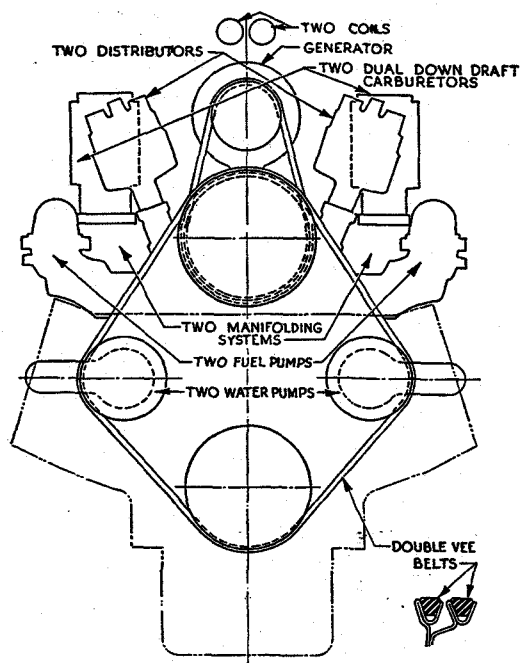
Dual Engine Accessories
