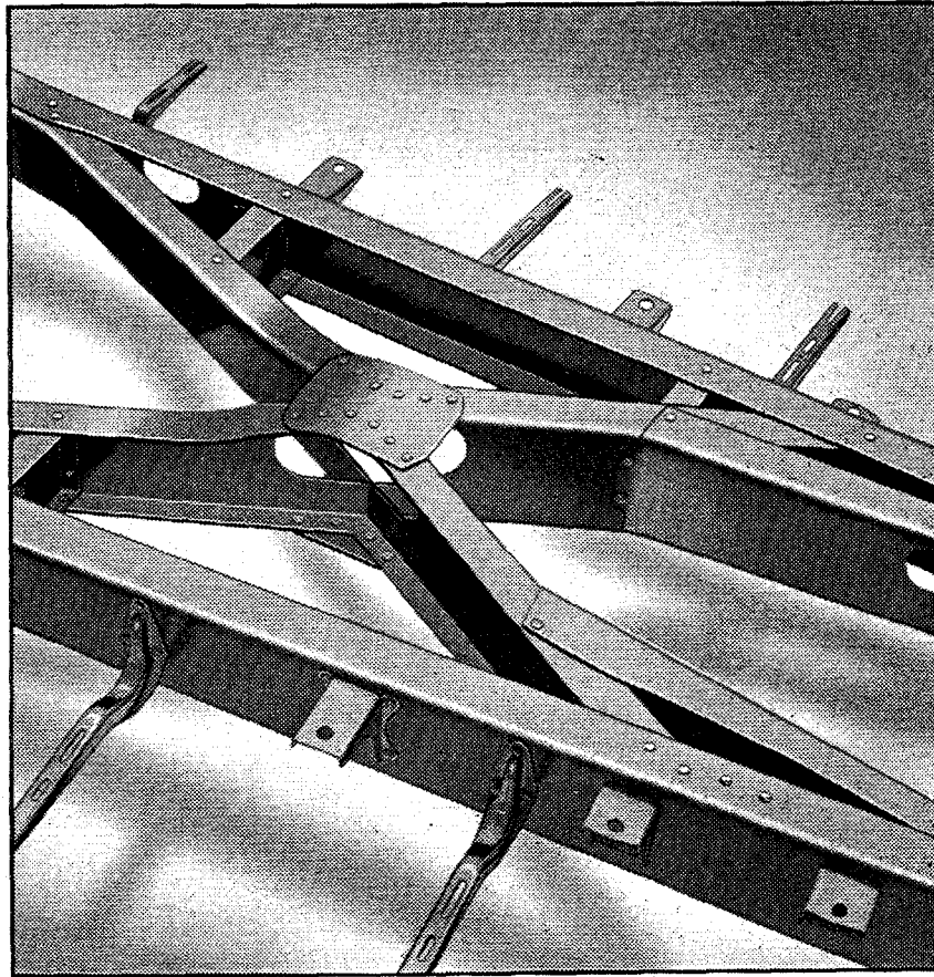
Heavy Fleetwood X-Type Channel Frame with Deep Center Junction
