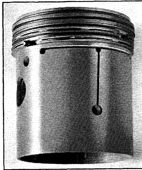
Anodized Aluminum Alloy, T-slot, 4-Ring Piston
