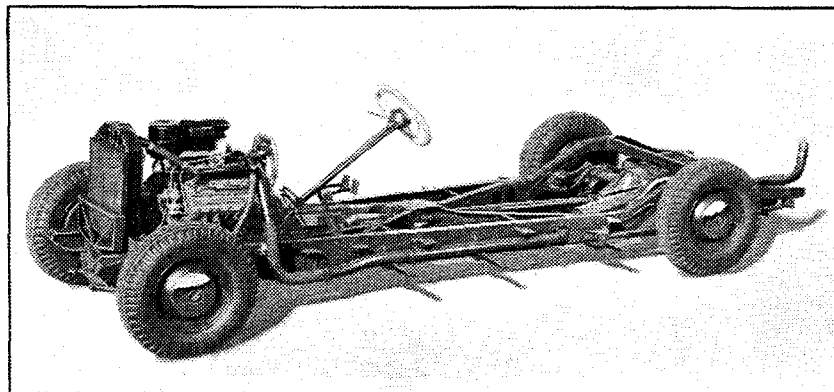
New Fleetwood V-8 Chassis
