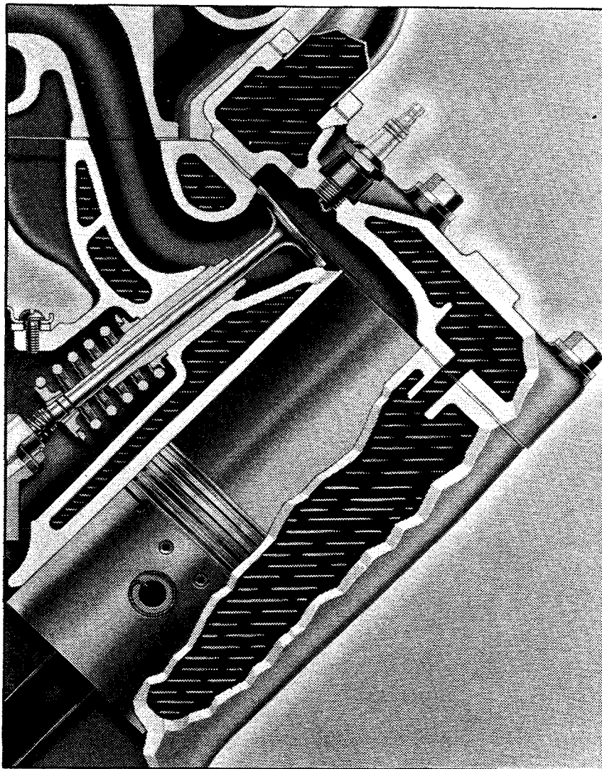
Full Length Water Jackets
