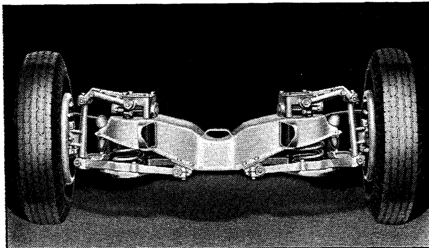
Cadillac Fleetwood Knee Action
