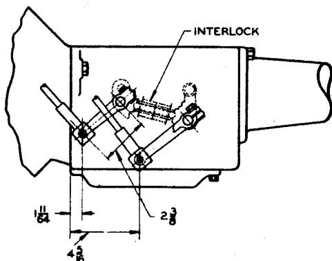
Fig. 10. Shifting mechanism at transmission case.
