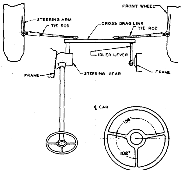
Fig. 15. Steering layout and connections, Series 39-50 and 61.
