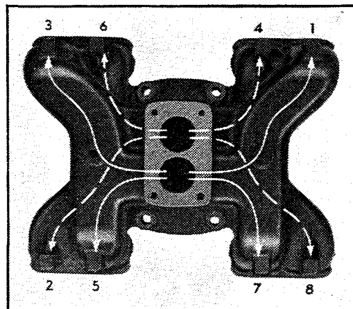
Equalized Manifolds
