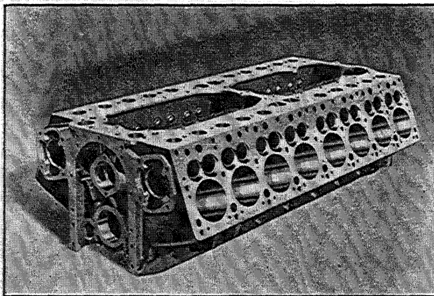
Enbloc Cylinder and Crankcase
