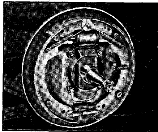
Cadillac Hydraulic Brake
