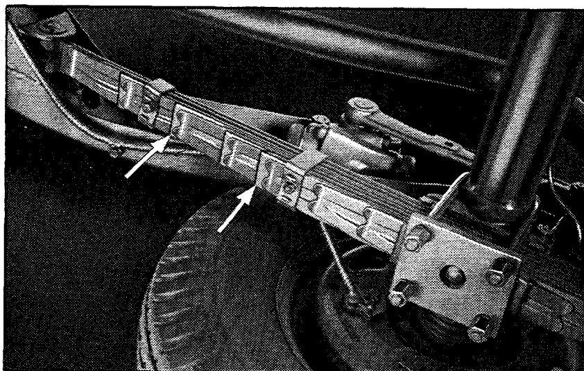
Rear Spring with Wax Liners
