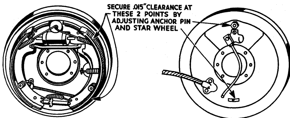
Fig. 6. Adjustment of brake shoes, Series 39-50, 61 and 60S.
