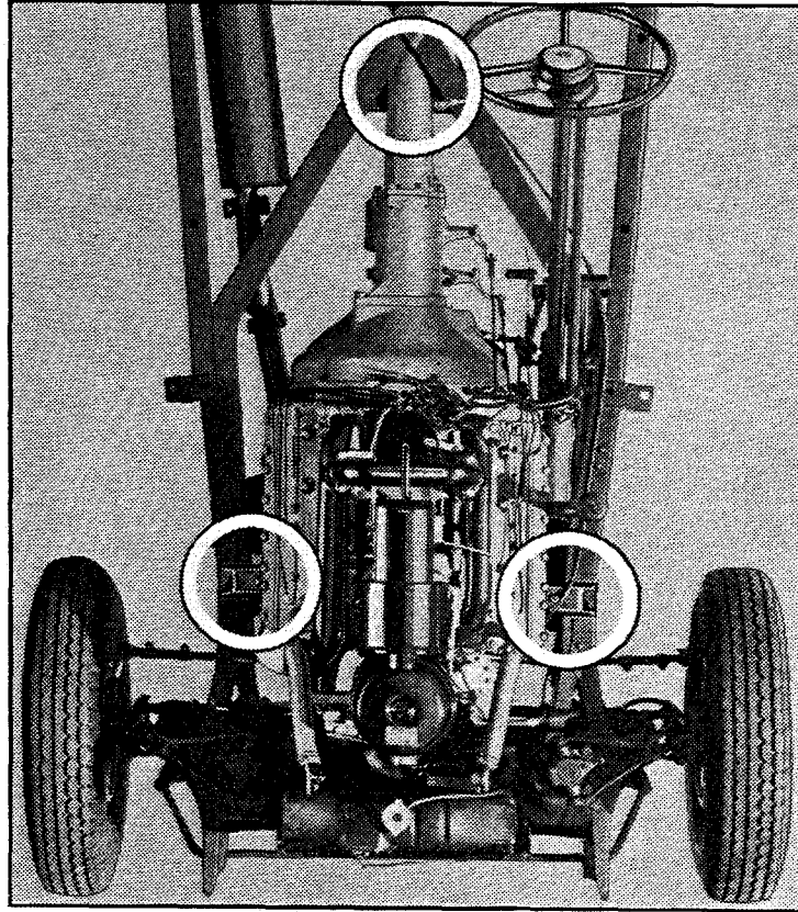
Cadillac-built V-8 Engines are Mounted at Three Points on Live Rubber
