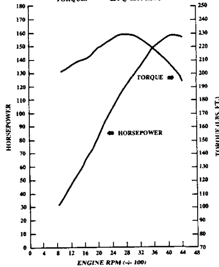
4.3L V6 RPO LB4 HORSEPOWER: 160 @ 4000 RPM TORQUE: 230 @ 2800 RPM
